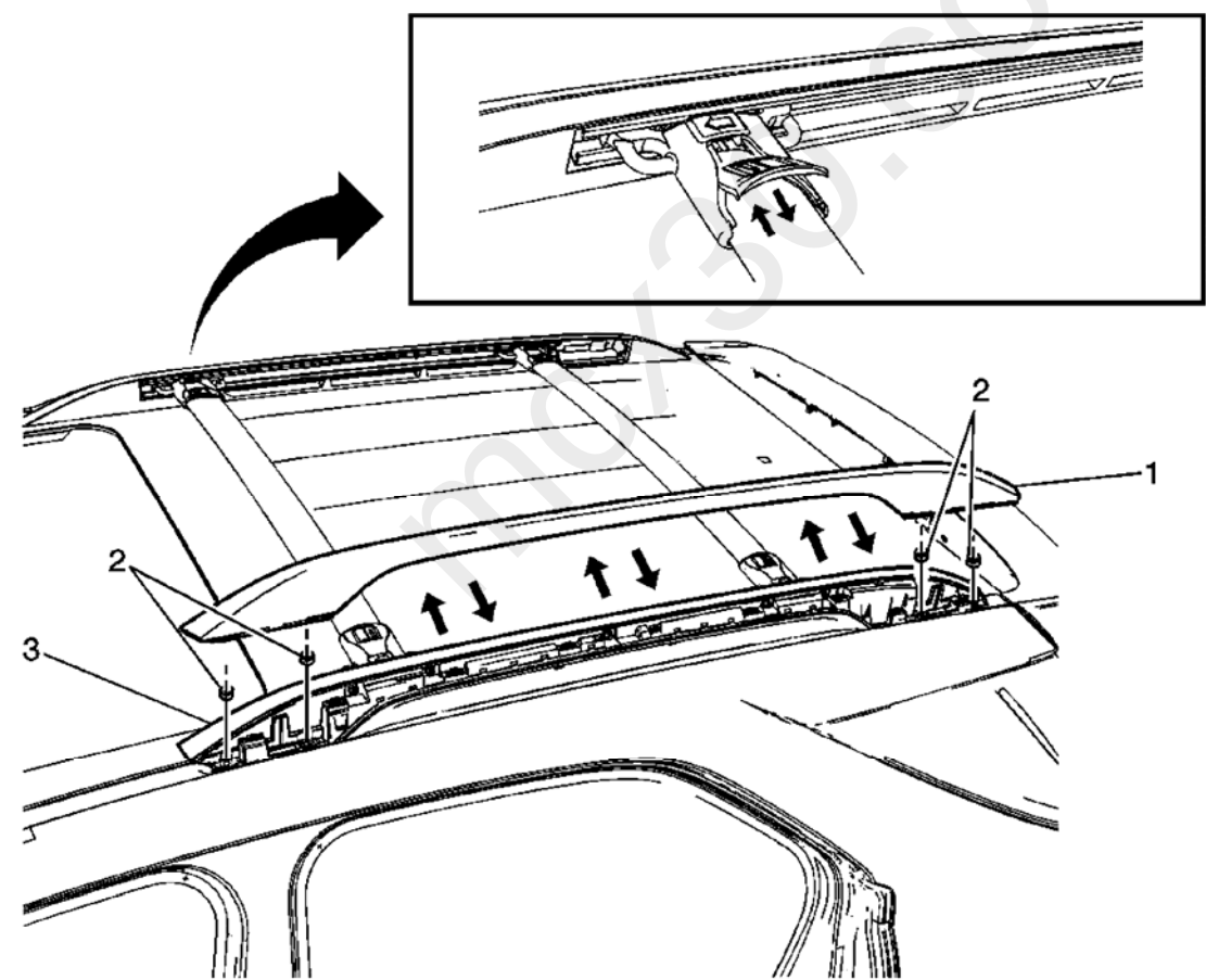
Fig. 1: Identifying Luggage Carrier Side Rail Components Courtesy of GENERAL MOTORS CORP.
